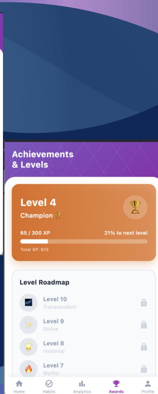
Fig 4. Achievements screen
