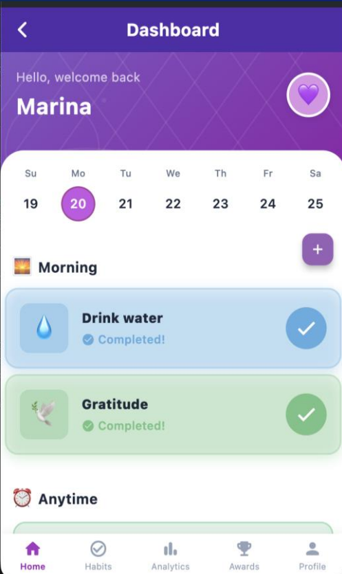
Fig 1. Dashboard Screen
