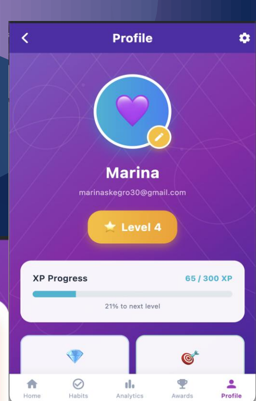
Fig 5. Profile Screen
