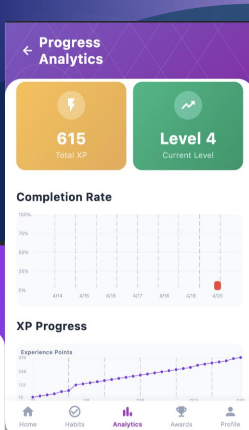
Fig 3. Analytics Screen
